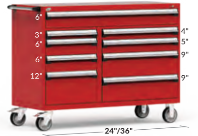
9 CAJONES R5GKE-3823 60" x 24" x 45½" R5GKG-3823 60" x 27" x 45½"
