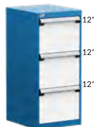
3 CAJONES L3ABD-4007__ 18" x 21" x 40" L3ABG-4007__ 18" x 27" x 40"
