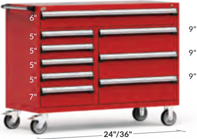
9 CAJONES R5GKE-3825 60" x 24" x 45½" R5GKG-3825 60" x 27" x 45½"
