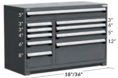
10 CAJONES R5KJE-3401 54" x 24" x 36" R5KJG-3401 54" x 27" x 36"
