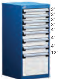
8 CAJONES L3ABD-4011__ 18" x 21" x 40" L3ABG-4011__ 18" x 27" x 40"
