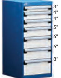
7 CAJONES L3ABD-4027__ 18" x 21" x 40" L3ABG-4027__ 18" x 27" x 40"
