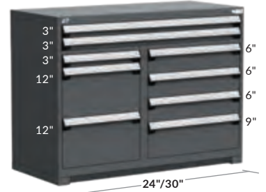
9 CAJONES R5KJE-3801 54" x 24" x 40" R5KJG-3801 54" x 27" x 40"
