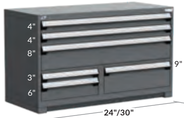
6 CAJONES R5KJE-3003 54" x 24" x 32" R5KJG-3003 54" x 27" x 32"
