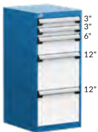
5 CAJONES L3ABD-4047__ 18" x 21" x 40" L3ABG-4047__ 18" x 27" x 40"
